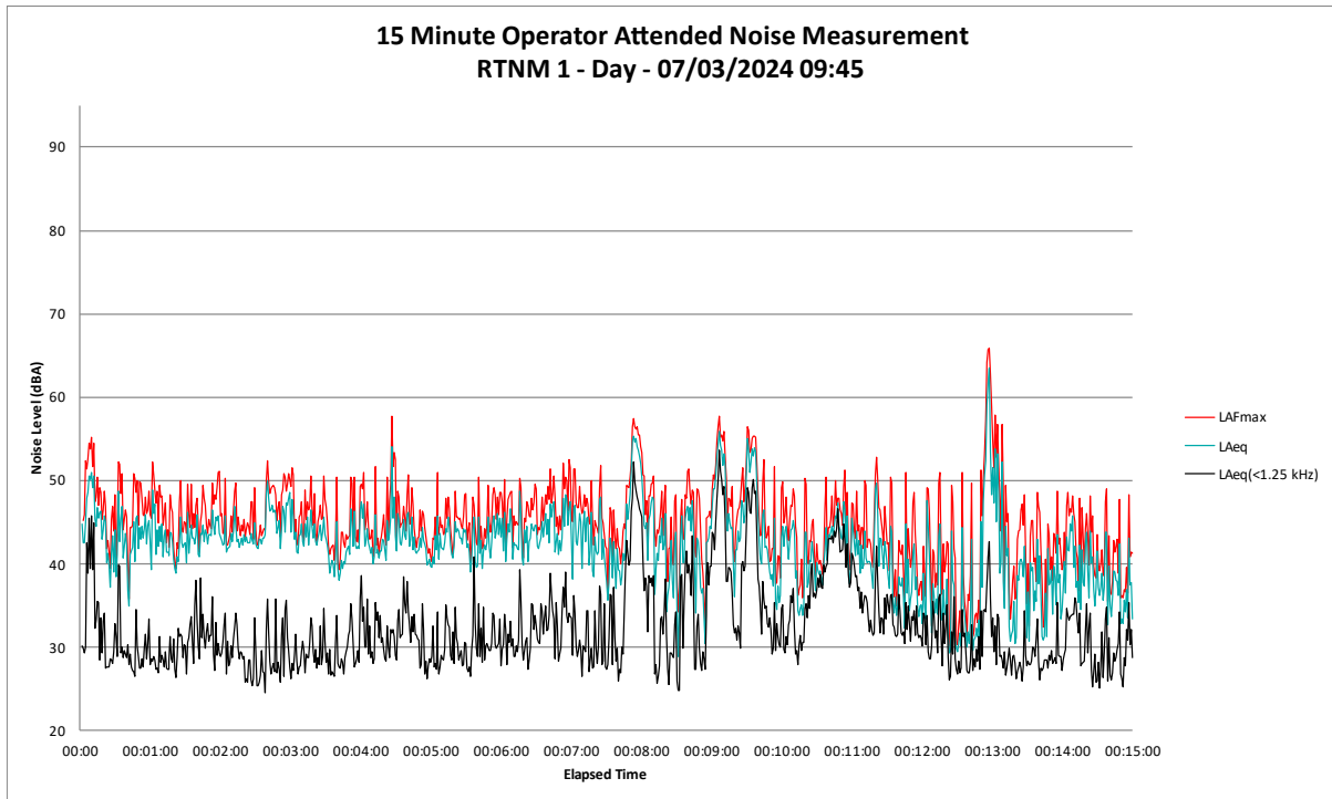
Figure B22 – ‘RTNM1’ Operator Attended Noise Survey Results
