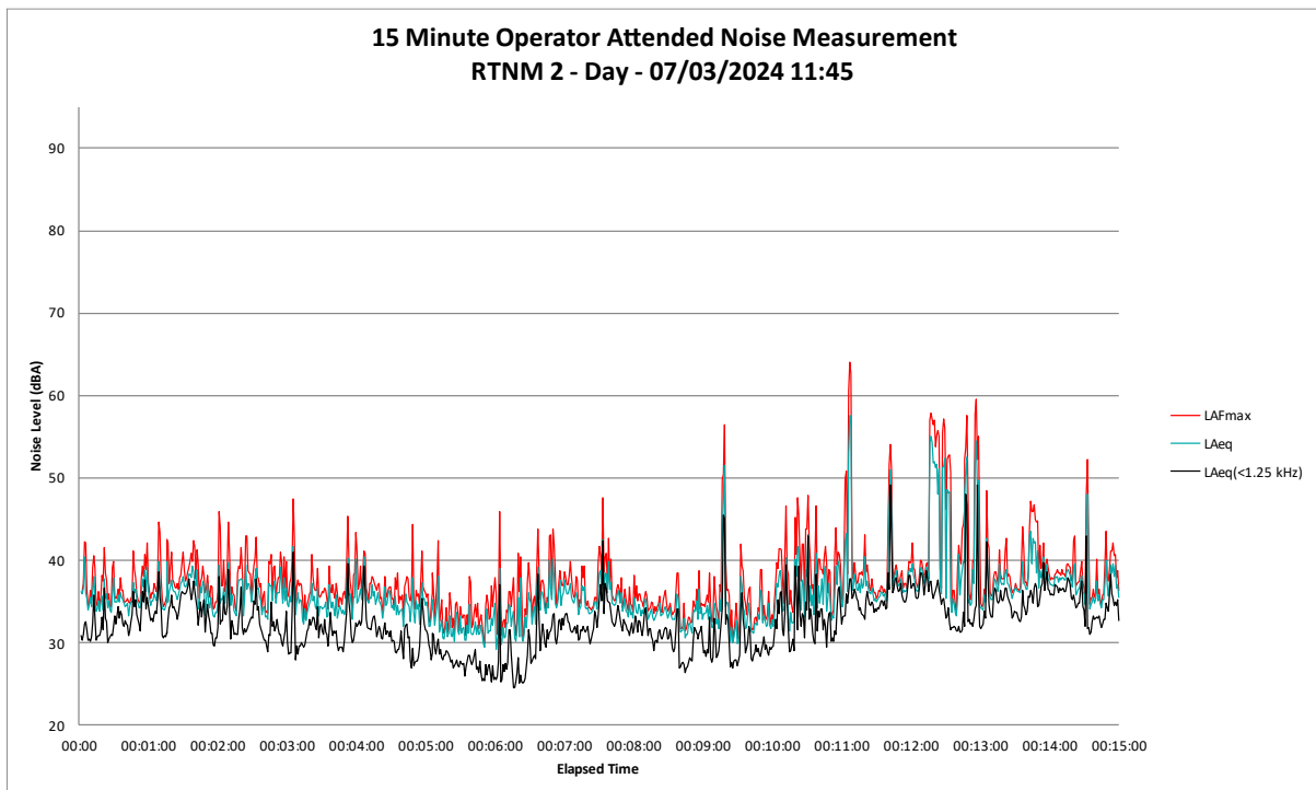
Figure B23 – ‘RTNM2’ Operator Attended Noise Survey Results
